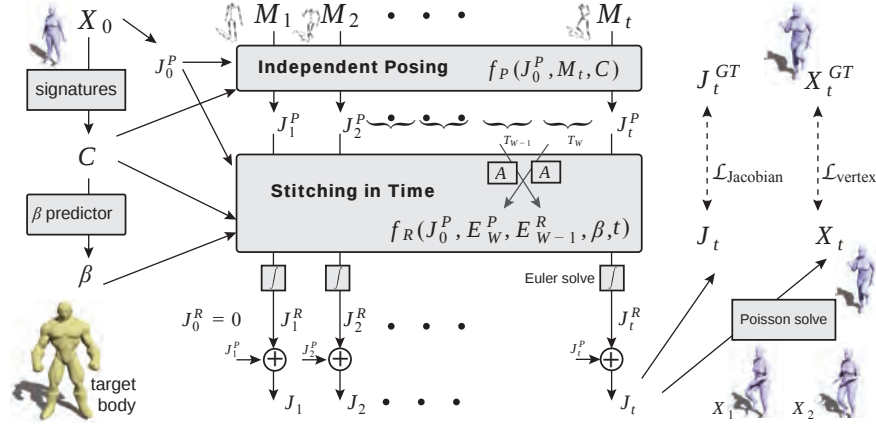
Fig. 2: Method overview. Starting from input stick figure motion ( \{M_i\} ) and a target body shape ( X_0 ), Residual Temporal Jacobians makes local predictions, using primary f_P and residual f_R MLPs, to predict spatial and temporal changes to per-triangle Jacobians. These are then integrated in space, via a Poisson solve, and in time, via numerical Euler stepping, to predict motion dynamics at time frame t . These two learnable modules are trained simultaneously with only direct object-level supervision using a combination of positional and Jacobian losses. We use the ground-truth meshes from AMASS to supervise the predictions. The time t input is positionally encoded.
