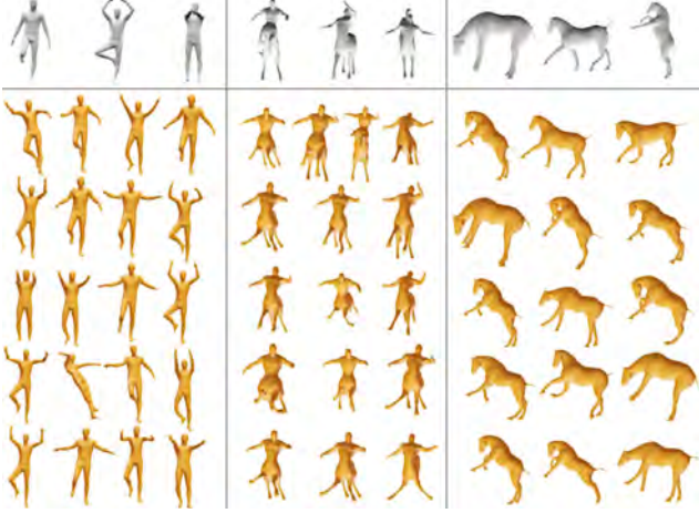
Figure 4: Training GLASS on the human, centaur, and horse meshes using the 3 examples each (top). (Bottom) We show random samples from the latent space, which combine different properties learned from the example deformations.
