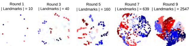
Figure 3: t-SNE embedding of generated samples shows progressive augmentation of the shape space. Sample color indicates originating (parent) shape. See also Fig. 1.
