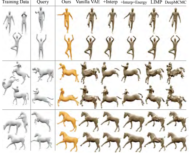
Figure 5: Generation results evaluated by coverage. We train different methods on the same training data (col 1) and generate comparable numbers of shapes. Given two shapes from the holdout data (col 2), we evaluate the methods by finding the closest generated shape (cols 3-8). Note how baseline techniques exhibit strong artifacts and usually do not generate a good match to the query shape.
