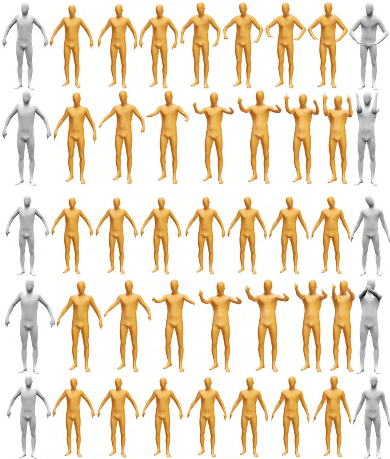
Figure 14: Faust-10 Interpolation results 1/6.
