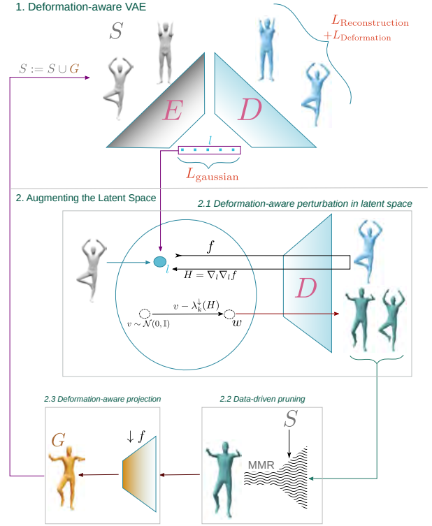
Figure 2: We present GLASS to iteratively build a deformation-aware VAE latent space and analyzing it to generate new training samples to augment the original training set. These enables generation of diverse yet plausible shape variations starting from very few input examples.
