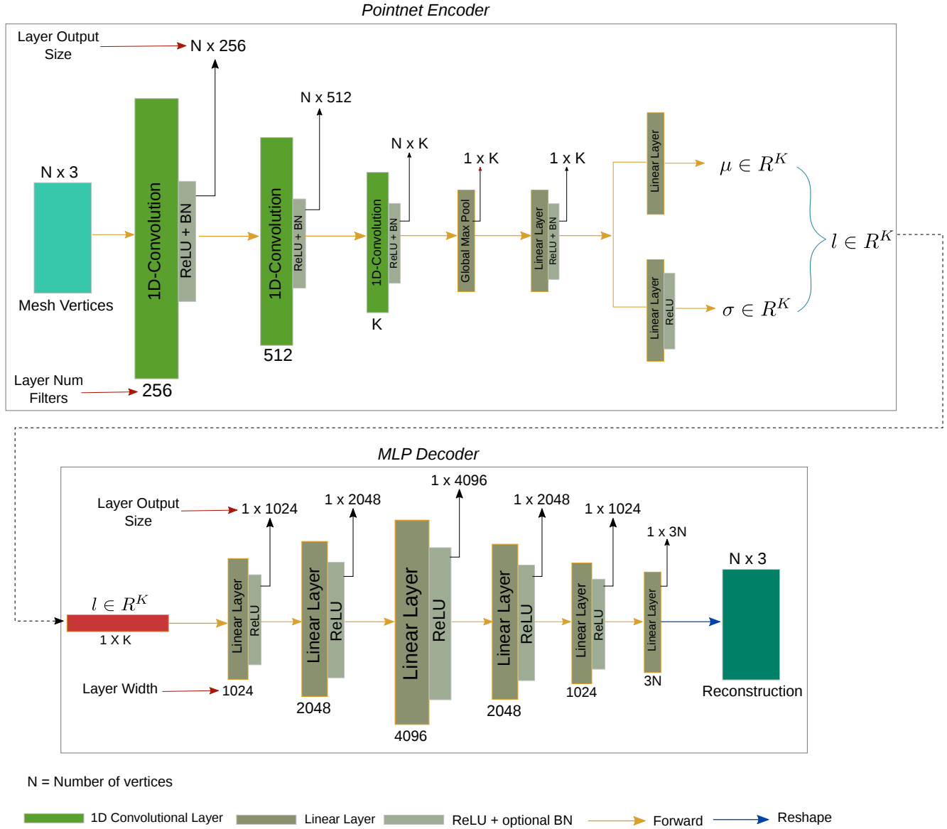
Figure 31: VAE network architecture: Pointnet Encoder (top) contains 3 convolutional layers (green) with ReLU/BN, followed by Global Max Pooling to obtain a feature for the set of vertices. The feature is input to a linear layer that further branches into 2 layers that output the gaussian parameters \mu and \sigma from which we sample the latent code to be input to the decoder. The decoder is a 5 layer fully-connected network that transforms the latent code to a 3N size output which is reshaped to N \times 3 to give us the reconstruction of vertices.
